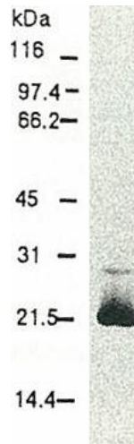
Fig. 1 Western blot of HCV core protein. Chimp liver cells were infected with recombinant vaccinia virus containing a HCV genome cDNA and were subjected to Western blot using this antibody. The core protein is detected as a 22kDa band.
